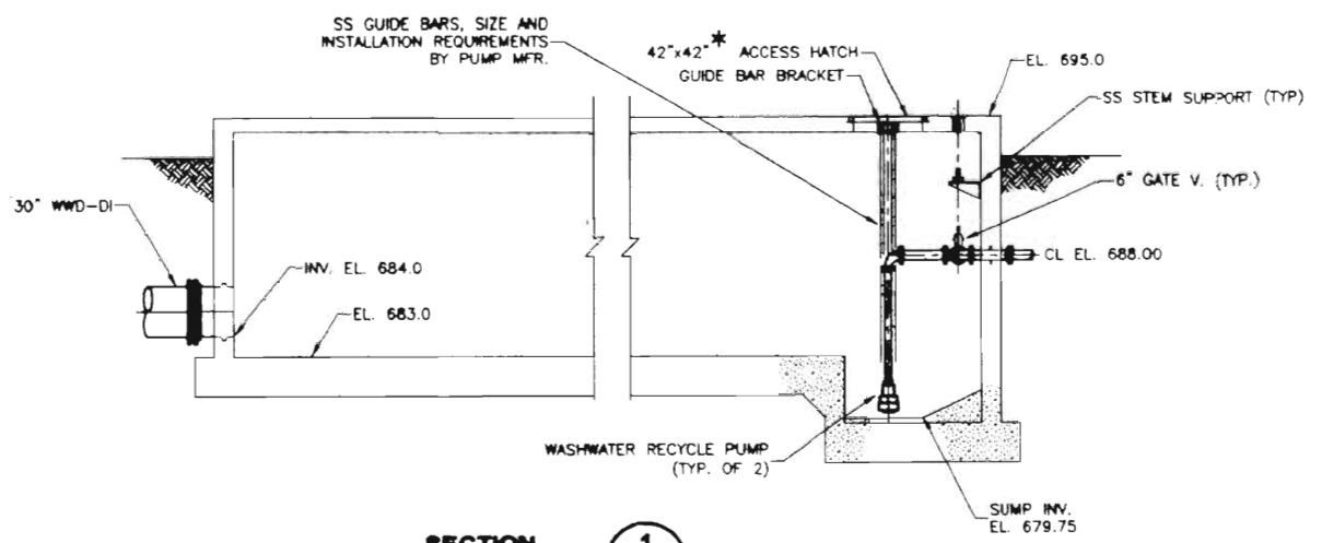
SECTION 1 3/16" = 1'-0"
