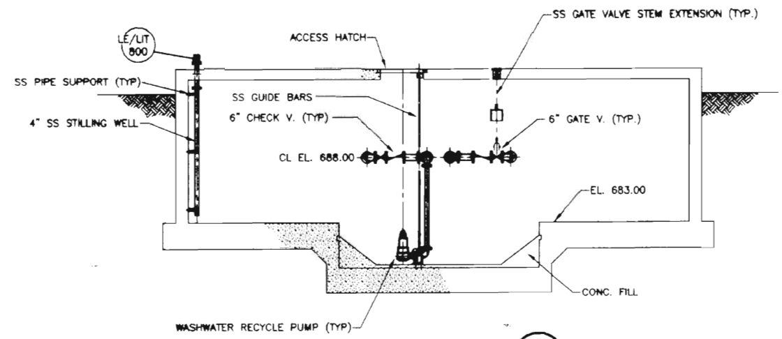
SECTION 2 3/16" = 1'-0"
