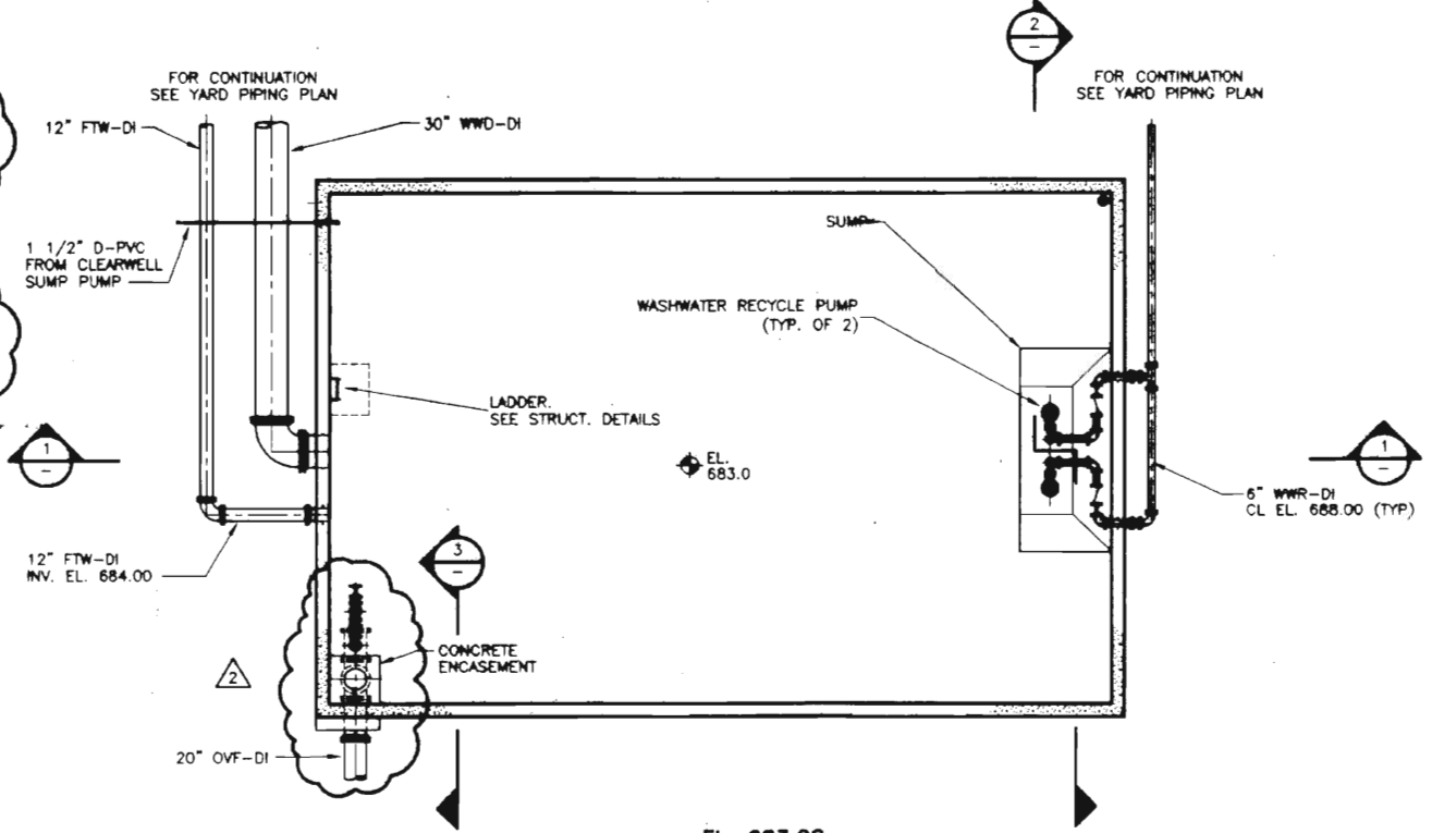
EL. 683.0 PLAN 1/8" = 1'-0"
