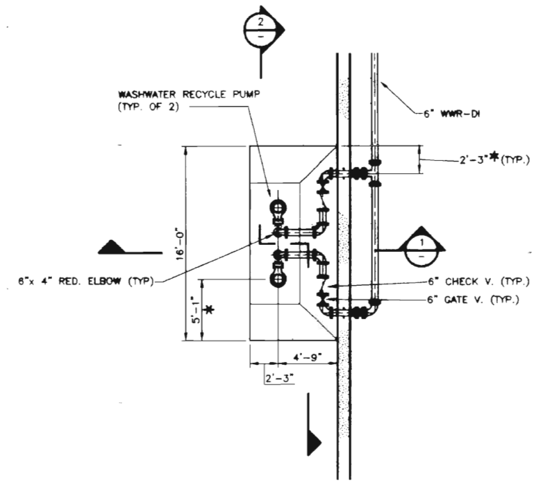
PART PLAN AT SUMP DETAIL A 3/16" = 1'-0"
