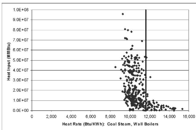
Figure 4. Coal Wall Boilers—Heat Input-Weighted Heat Rates
