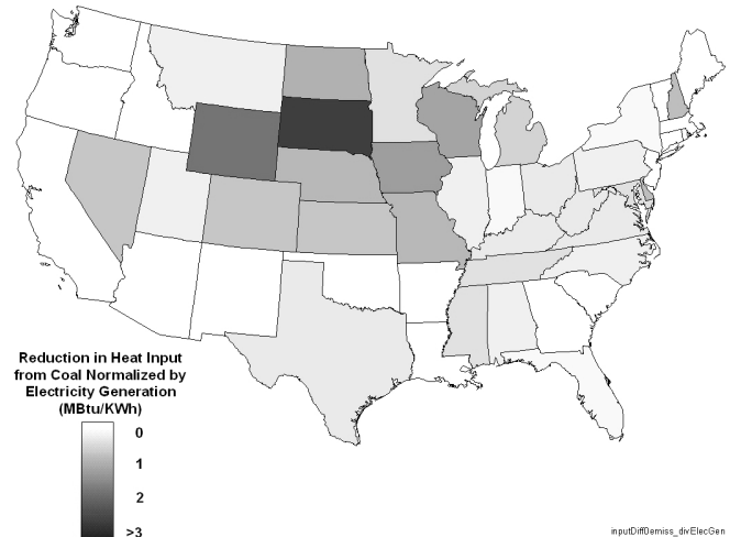
Figure 9. Coal Plants—Strict 5% Greater Efficiency Performance Standard
